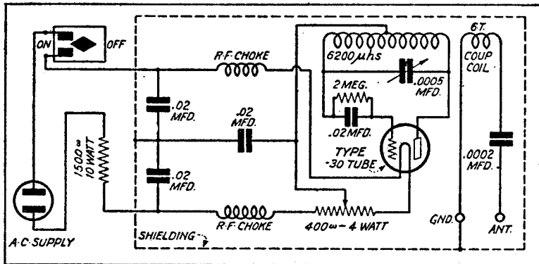
Model 60 Oscillator
